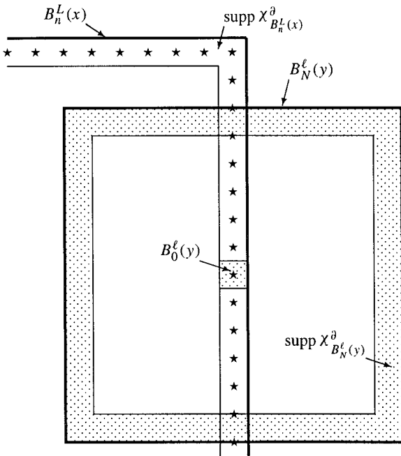
Fig. 3. Sketch of the geometric situation on the frame of B_n^L(x) for 1 \leq n \leq N-1 and d=2 . The points marked by \star make up the set T_n^L(x) and are the centres of the “tiling” of the frame of B_n^L(x) . For one y \in T_n^L(x) the boxes B_0^\ell(y) and B_N^\ell(y) are sketched.
